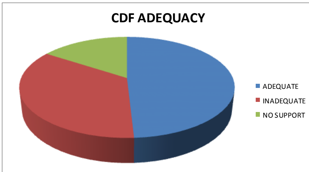
Fig. 1- Adequacy of CDF support
